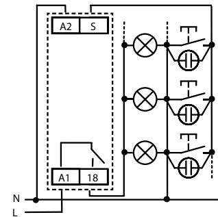
4-wire connection
