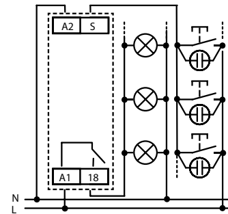
4-wire connection
