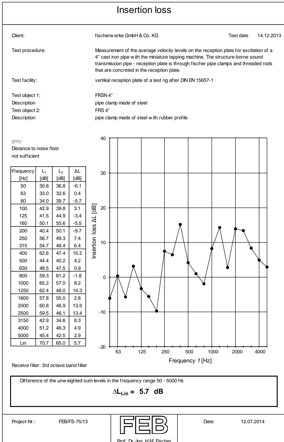
Figure 3: Insertion loss of the pipe clamp FRS 4"
