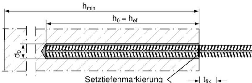
Reinforcing bar
